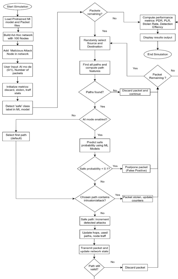
Figure 2 Proposed Flowchart
