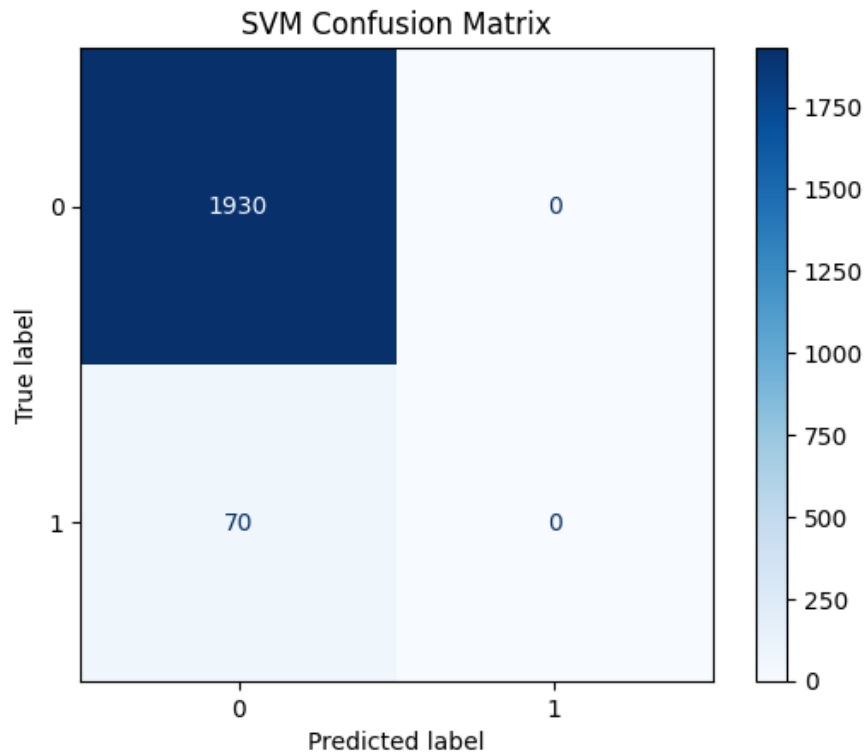
Figure 11 Confusion Matrix
