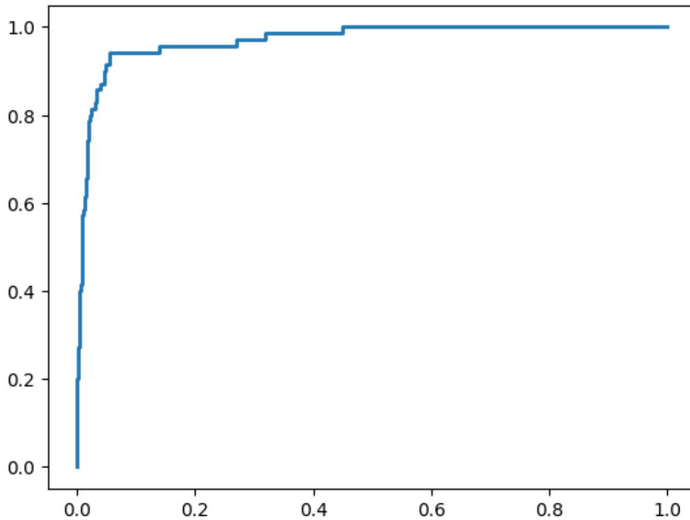
Figure 19 svm
