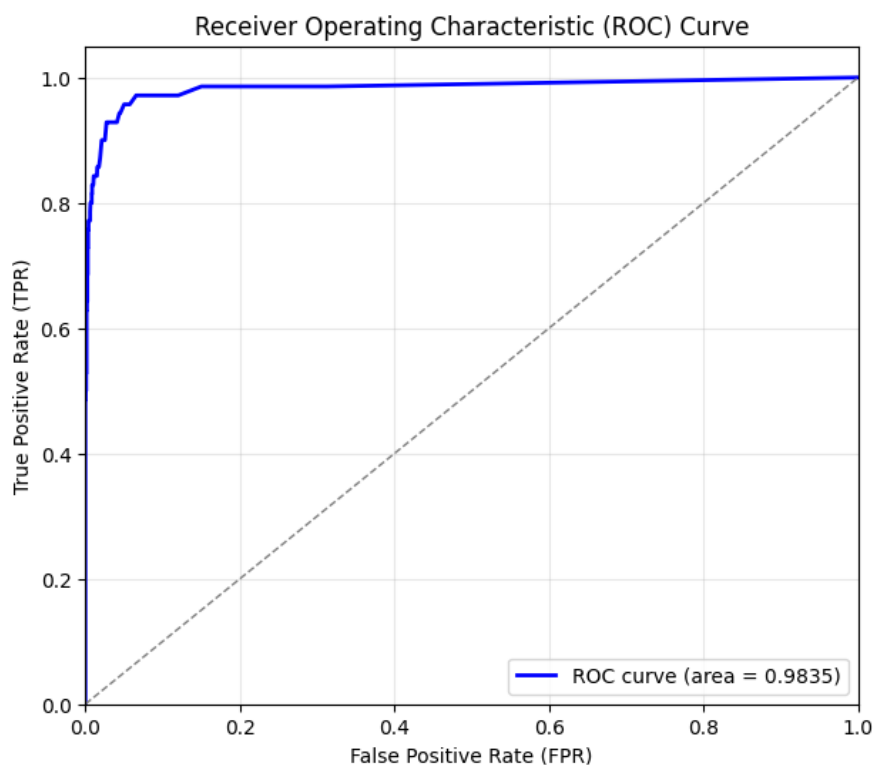
Figure 8 RANDOM FOREST
