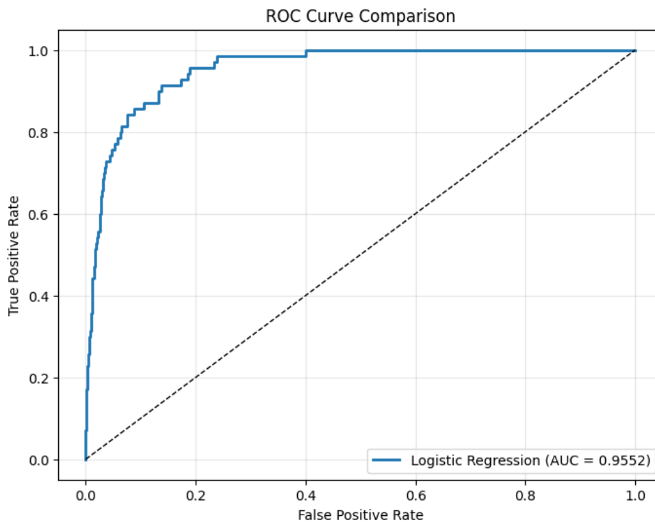
Figure 21 logistic regression
