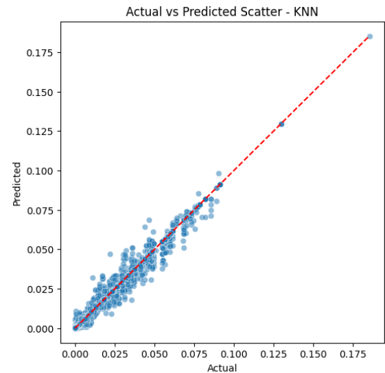
Fig. 10 Actual vs Predicted Scatter Plot-KNN
