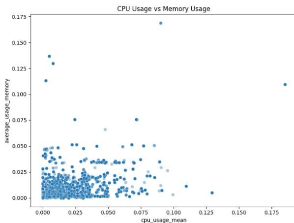
Fig. 2 Scatter Plot of CPU Usage vs Memory Usage
