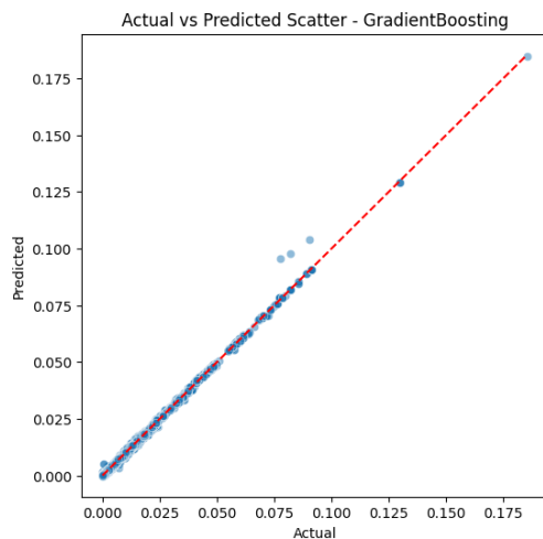
Fig. 12 Actual vs Predicted Scatter Plot-Gradient Boosting
