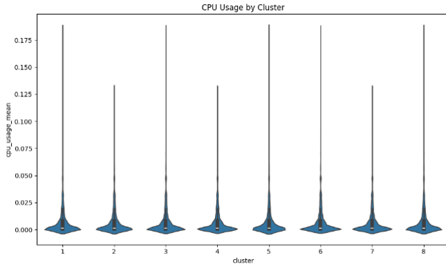
Fig. 7 Cluster-Level CPU Usage Differences
