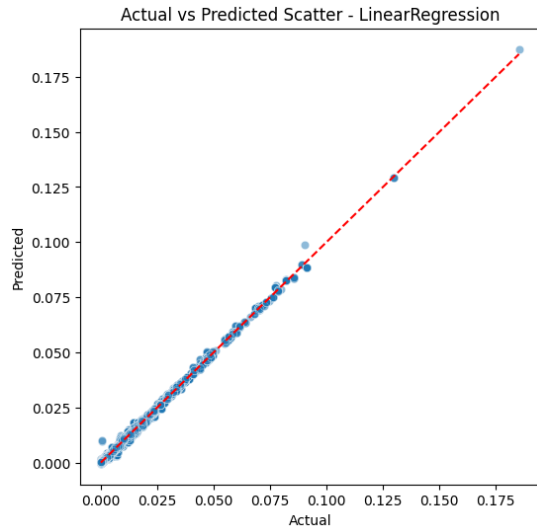
Fig. 11 Actual vs Predicted Scatter Plot-Linear Regression
