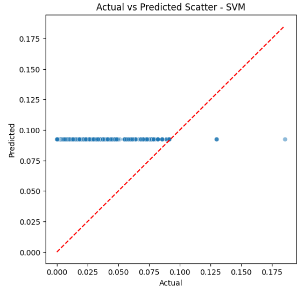
Fig. 9 Actual vs Predicted Scatter Plot-SVM
