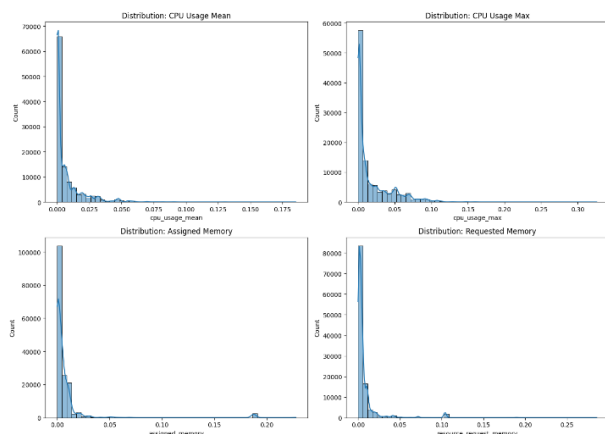
Fig. 4 Distribution of Usage Metrics
